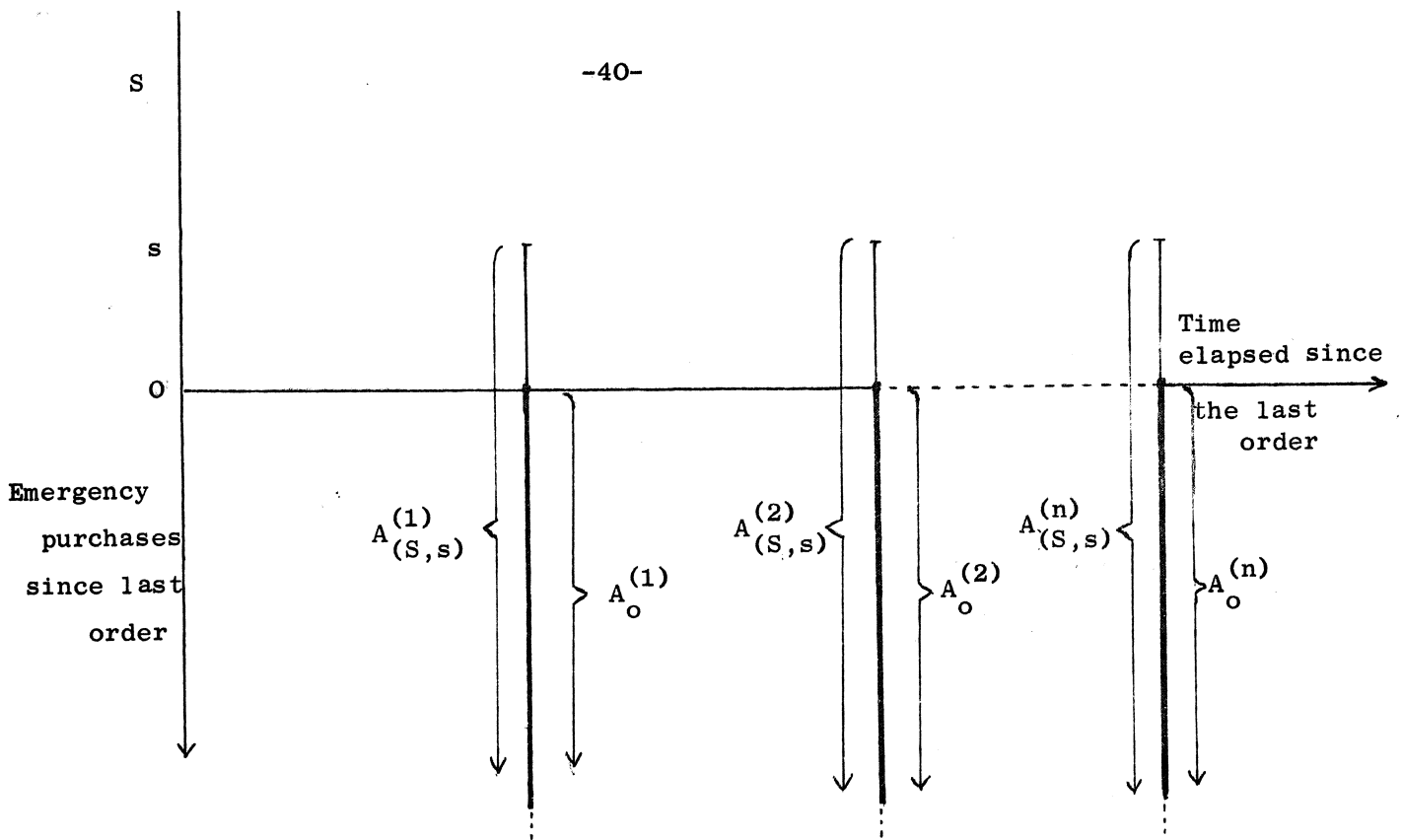
fig.1 The state space \psi
